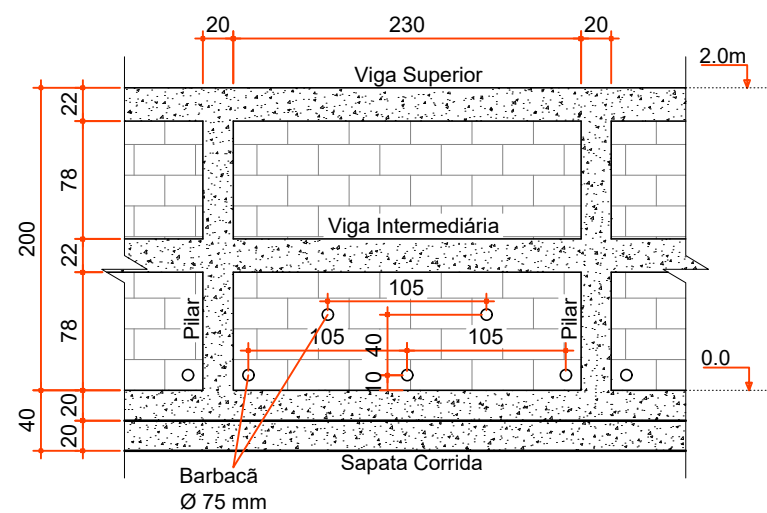
VISTA FRONTAL
