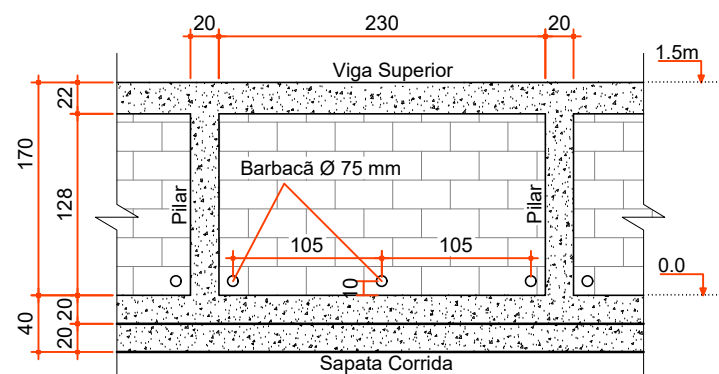
VISTA FRONTAL
