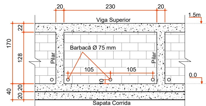
VISTA FRONTAL
